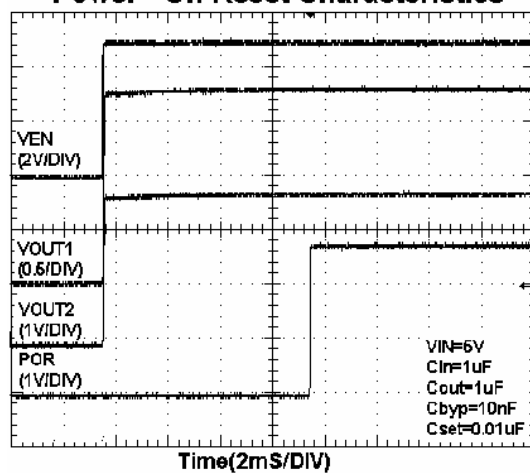
Power - On Reset Characteristics
