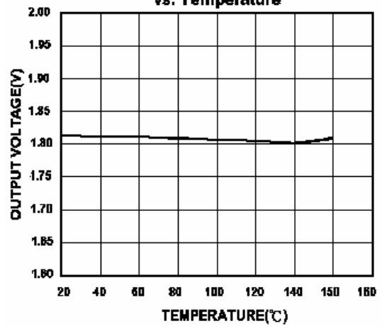
Output Voltage 1 vs. Temperature
