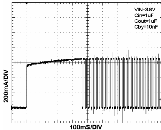
CURRENT LIMIT OUT2
