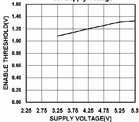
Enable Voltage Threshold vs. Supply Voltage
