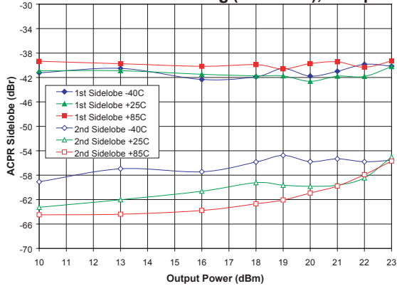
Figure 14: ACPR 1st & 2nd Sidelobes vs. Output Power Across Temp. (Freq = 2.45GHz, V CC = +3.3V) 802.11b Gaussian Filtering (BT = 0.45), 1 Mbps
