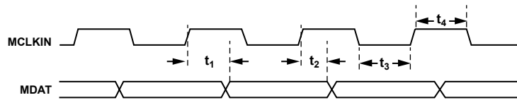
Figure 3. Data Timing
