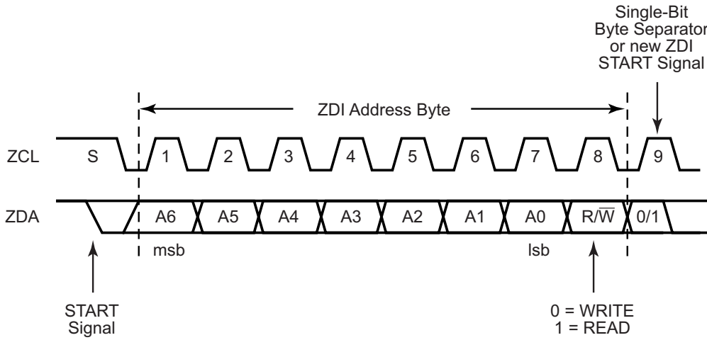
Figure 39. ZDI Address Write Timing
