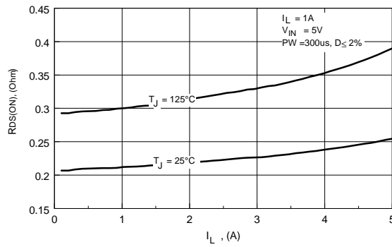
Figure 4. R_{DS(ON)} Versus I_L at V_{IN}=5.0\text{V} .
