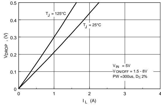
Figure 2. V_{DROP} Versus I_L at V_{IN}=5.0\text{V} .
