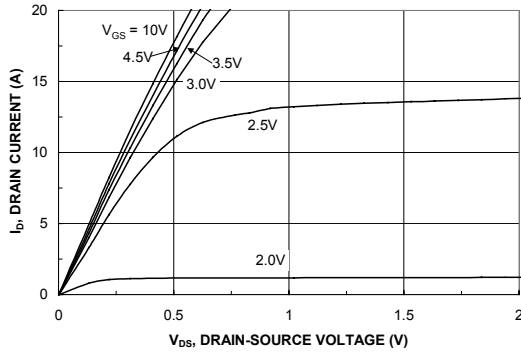
Figure 1. On-Region haracteristics.
