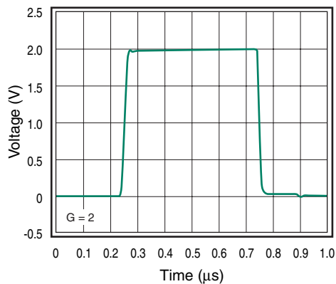
Figure 24. Large Signal Pulse Response ( \pm 5\text{V} )
