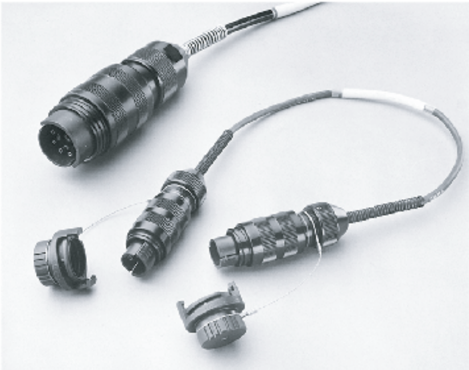
State-of-the-art ceramic alignment tips on the contact provide maximum coupling performance - less than 1.0 dB average coupling loss.
