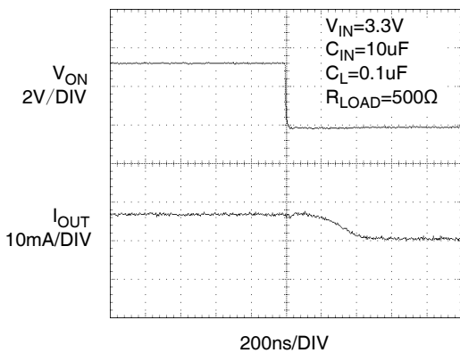
Figure 17. T OFF Response
