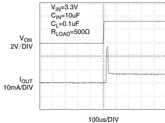
Figure 16. T ON Response
