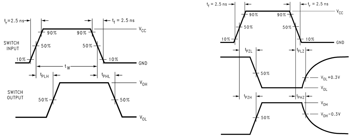
FIGURE 2. AC Waveforms
