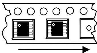
Feed Direction Typical SOP/MSOP Package Orientation
