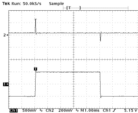
Line Transient
