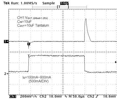
Load Transient
