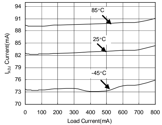
I ADJ Current vs. Load Current
