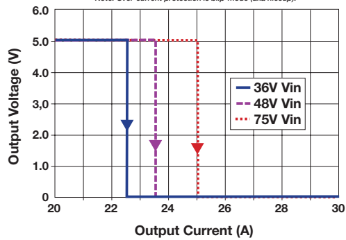
Over-current Protection
