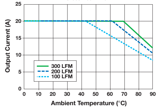
Thermal Derating Crosswise Airflow
