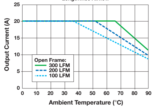
Thermal Derating Lengthwise Airflow
