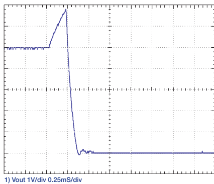
Over Voltage Protection
