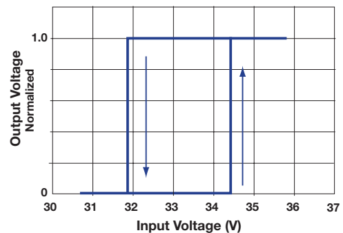
Undervoltage Hysteresis
