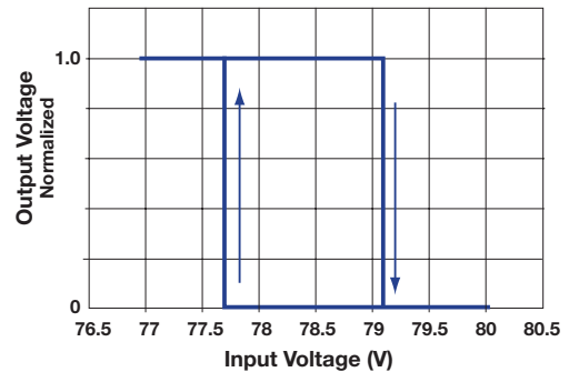
Overvoltage Hysteresis
