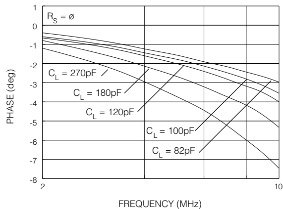
Fig. 4 Phase vs Frequency
