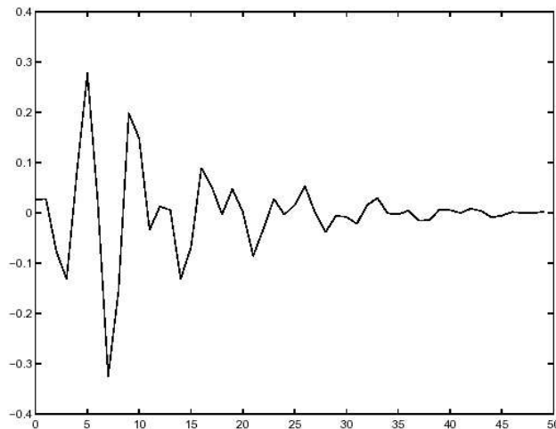
Figure 10. Minimum Phase Cancel Pulse Impulse Response, CANCEL_DELAY = 7
