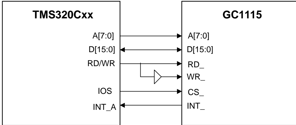
Figure 8. TMS320Cxx – GC1115 Interface
