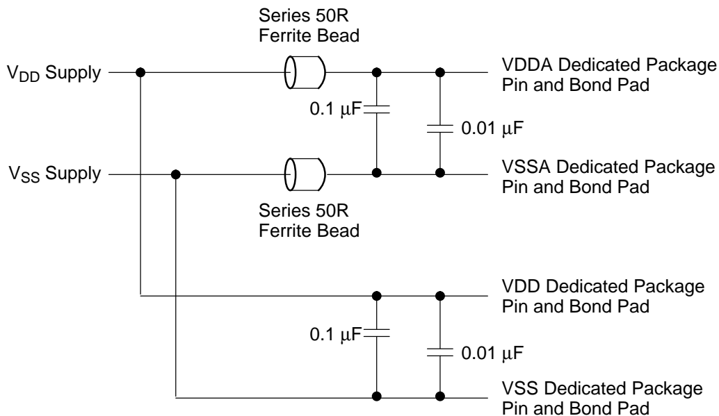
Figure 18. Power-Supply Filter
