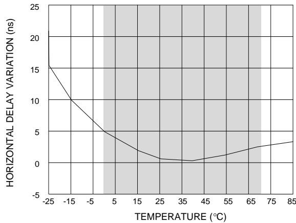
Fig. 11 Horizontal Delay Variation vs Temperature
