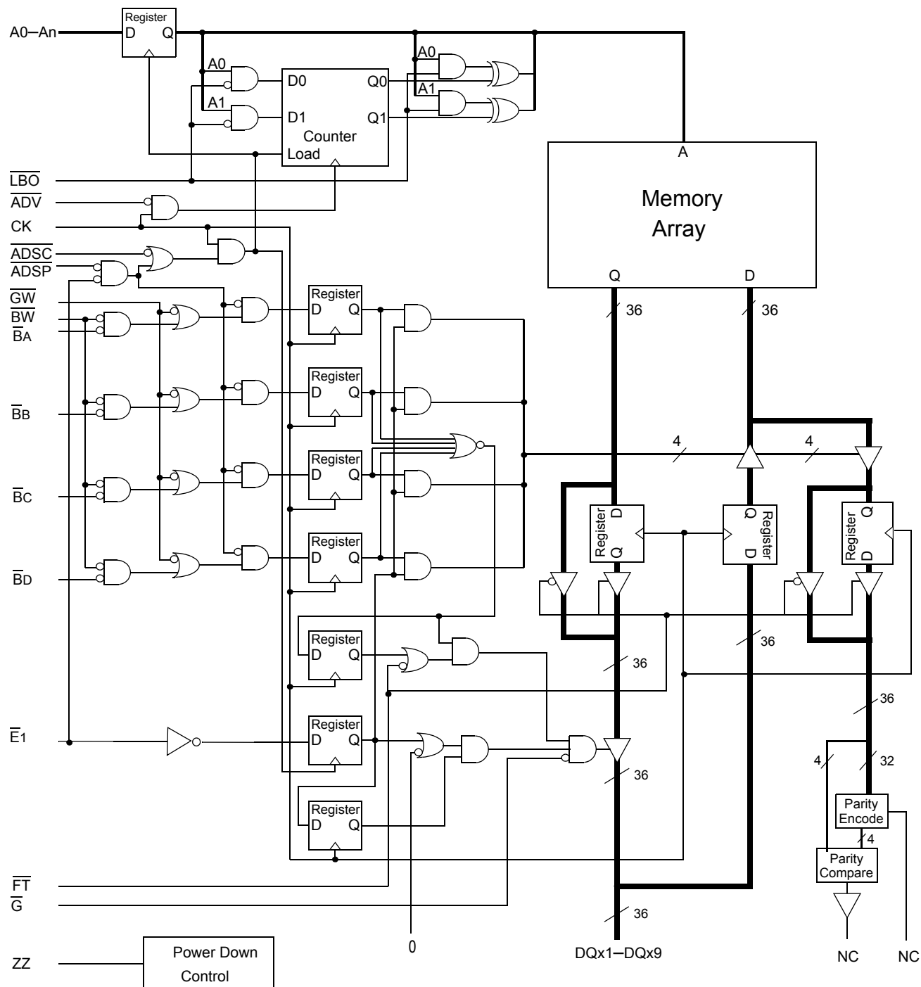
GS8321E18/32/36 Block Diagram
