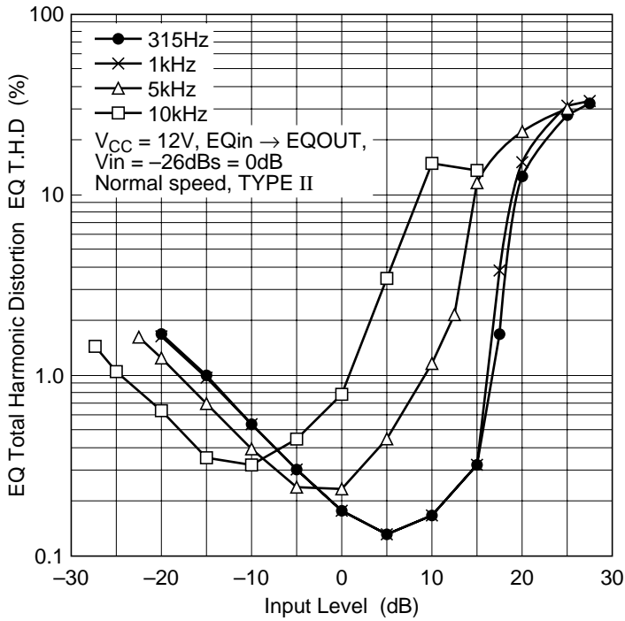
EQ Total Harmonic Distortion vs. Input Level (2)
