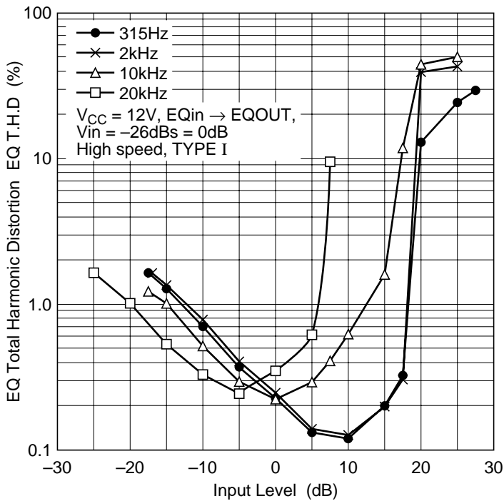
EQ Total Harmonic Distortion vs. Input Level (3)
