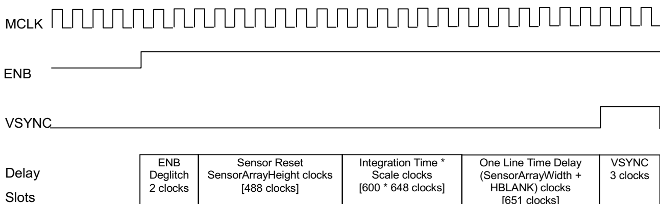
Fig. 5 Initial Data Setup Time after ENB gets active
