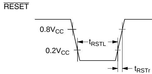
Figure 68 \overline{RESET} Timing
