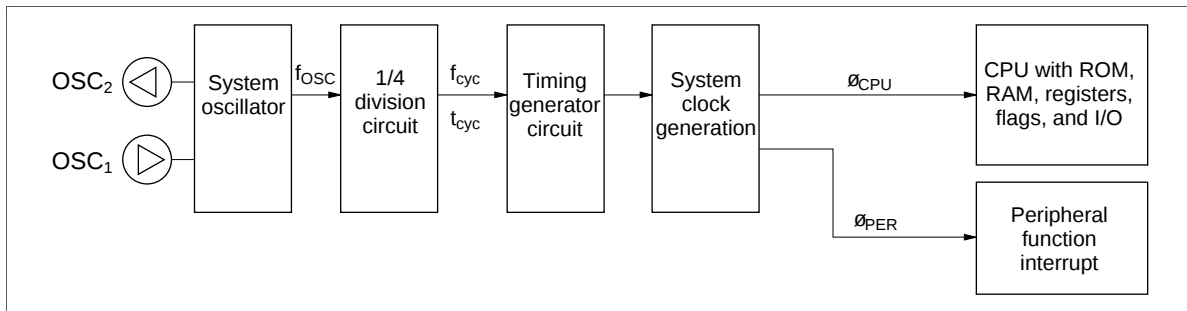
Figure 17 Clock Generation Circuit
