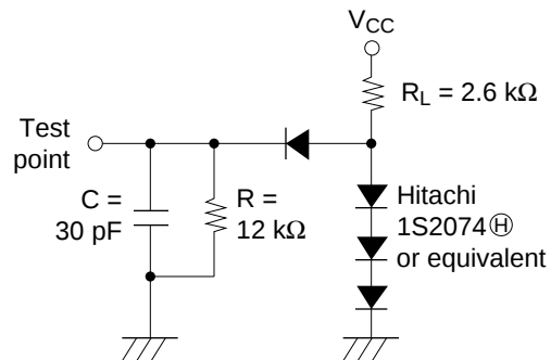
Figure 71 Timing Load Circuit
