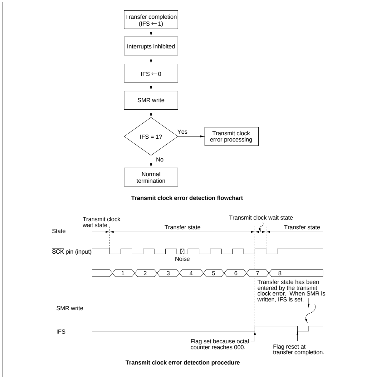
Figure 44 Transmit Clock Error Detection
