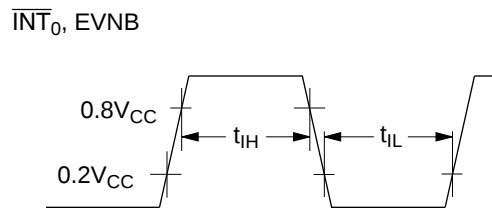
Figure 67 Interrupt Timing
