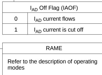
Figure 57 I AD Off Flag (IAOF)
