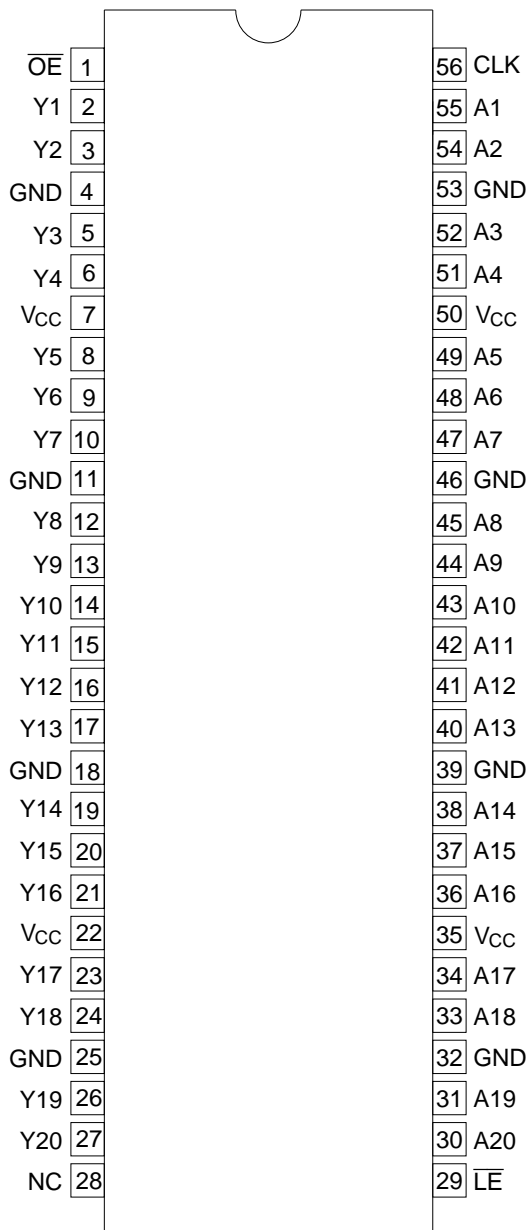
(Top view)
