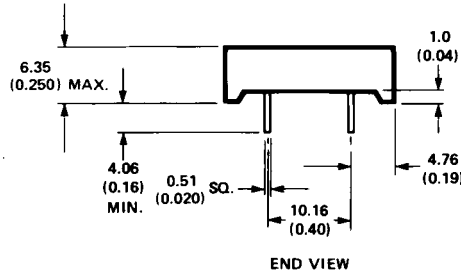
END VIEW
