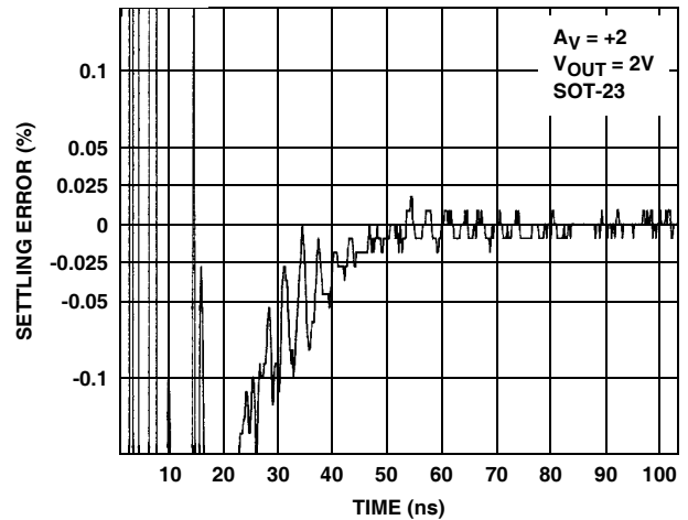
FIGURE 23. SETTLING RESPONSE
