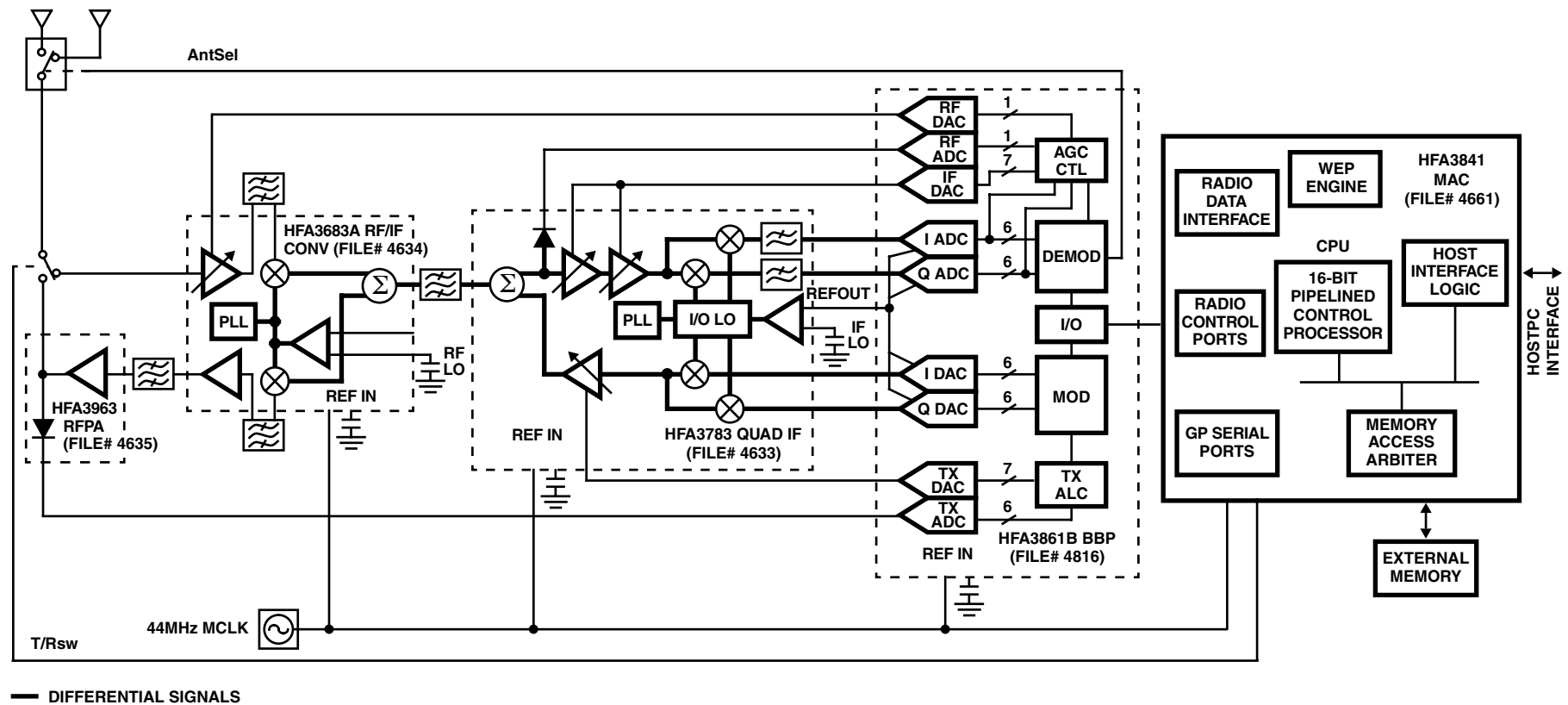
TYPICAL TRANSCEIVER APPLICATION CIRCUIT USING THE HFA3861B
