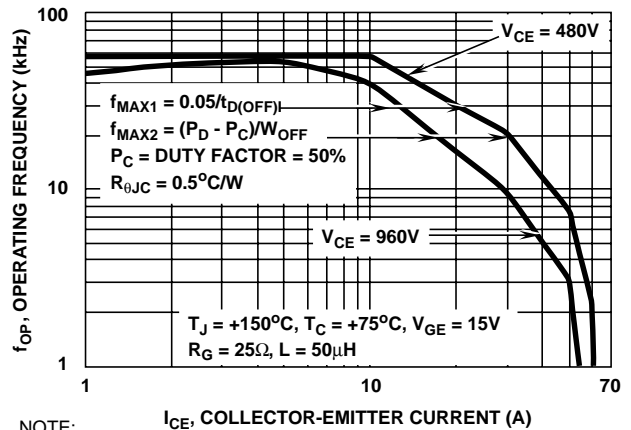
NOTE: I_{CE} , COLLECTOR-EMITTER CURRENT (A) P_D = ALLOWABLE DISSIPATION P_C = CONDUCTION DISSIPATION
