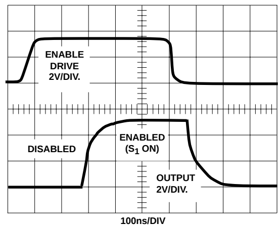
FIGURE 7C. WAVEFORMS
