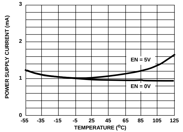
FIGURE 10B. HI-508/HI-509
