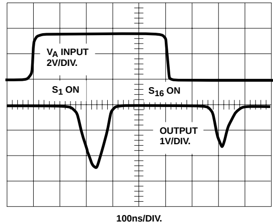
FIGURE 6C. WAVEFORMS
