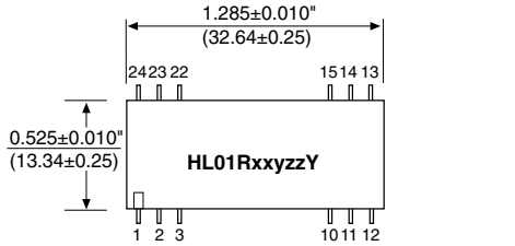
TOP VIEWS
