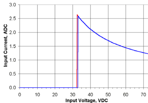
Fig. 6 HLS030ZD (2.5V) Input Characteristic
