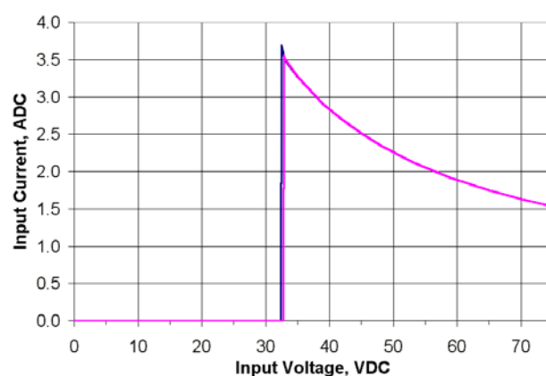
Fig. 5 HLS30ZE (3.3V) Input Characteristic
