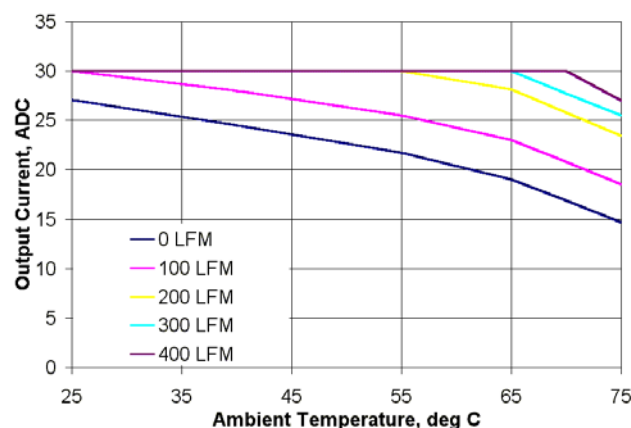
Fig.11 HLS30ZE (3.3V) derating curves
