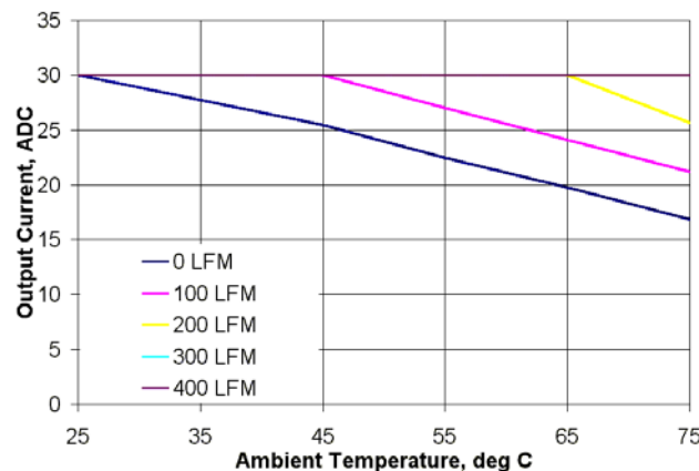
Fig.12 HLS30ZD (2.5V) derating curves
