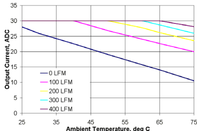
Fig.10 HLS30ZG (5V) derating curves
