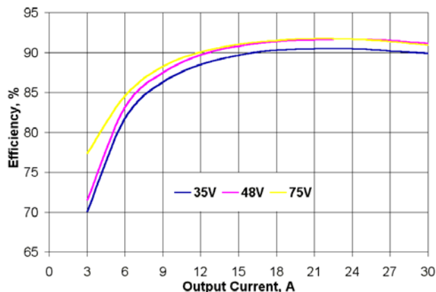
Fig. 1 HLS30ZG (5V) Efficiency vs. Output Load
