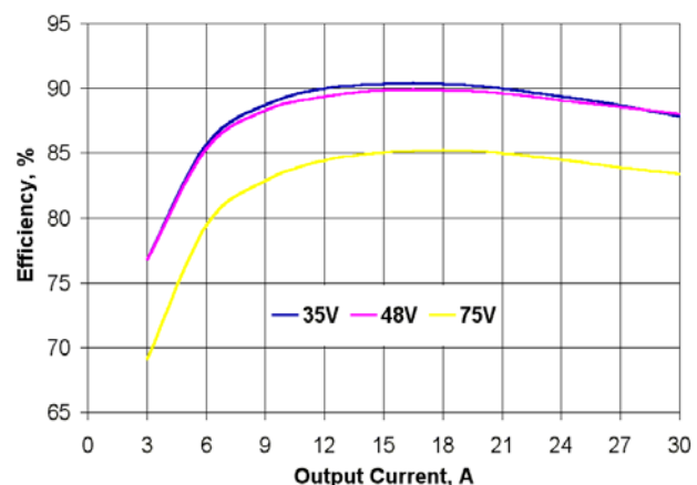
Fig. 3 HLS30ZD (2.5V) Efficiency vs. Output Load
