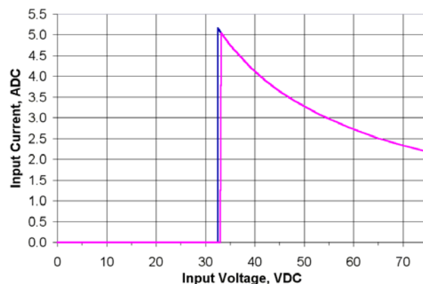
Fig. 4 HLS30ZG (5V) Input Characteristic
