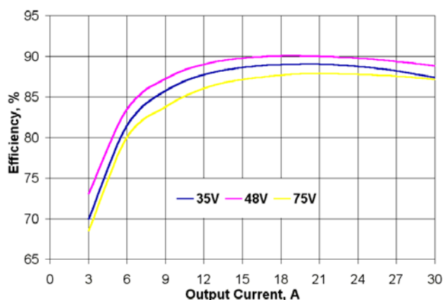
Fig. 2 HLS30ZE (3.3V) Efficiency vs. Output Load
