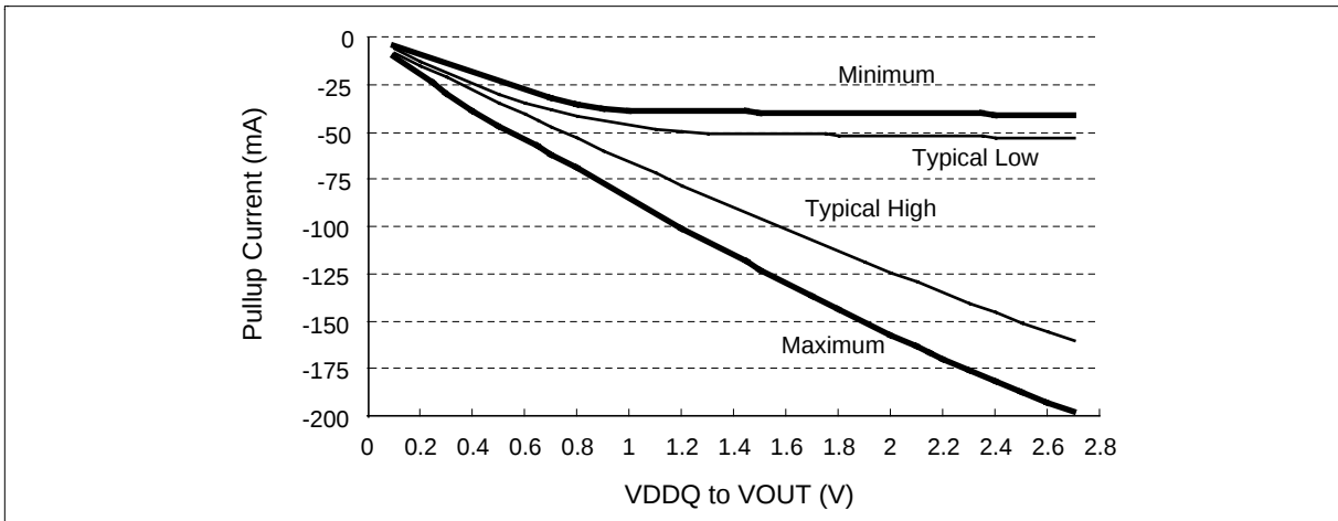
Pull-up Characteristics
