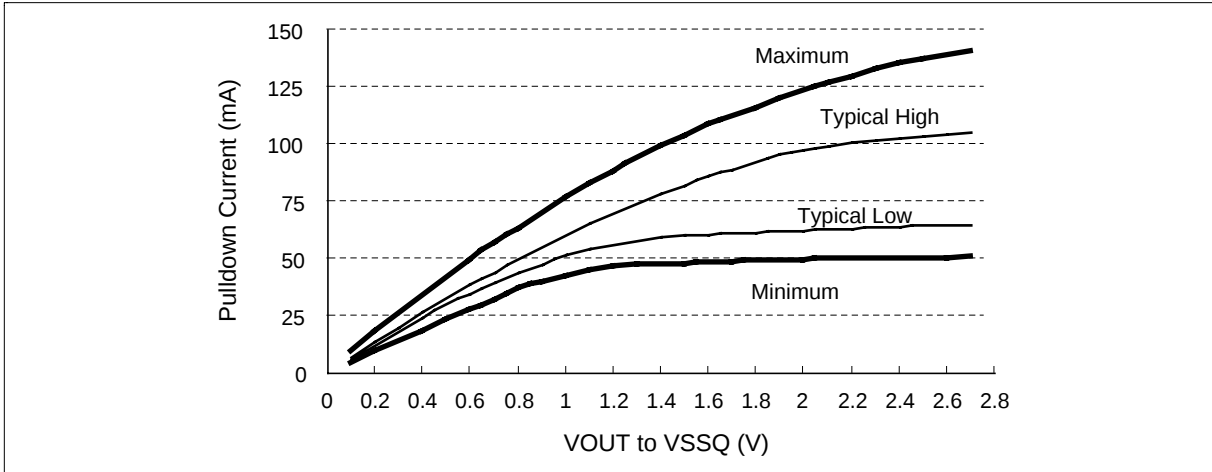
Pull-down Characteristics
