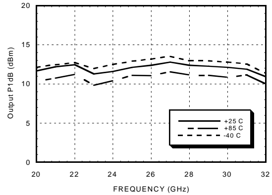
P1dB Output Power vs. Temperature @ Vdd= +4V
