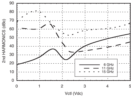
Second Harmonics vs. Control Voltage, Pin = -10 dBm
