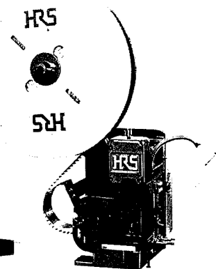
Auto Crimp Tool CM-105
