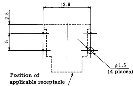
HR12-10R-SP (Stopper plate) (Applicable PCB thickness range 1~2)
