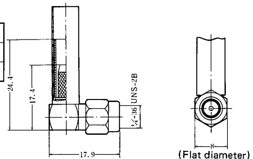
L-type Plugs for RG-142B/U and 3D-2W (Irrax cables)
