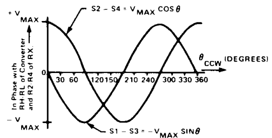
Standard Synchro Control Transmitter (CX) Outputs as a Function of CCW Rotation From Electrical Zero (EZ).
