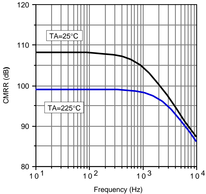
COMMON MODE REJECTION RATIO vs. FREQUENCY
