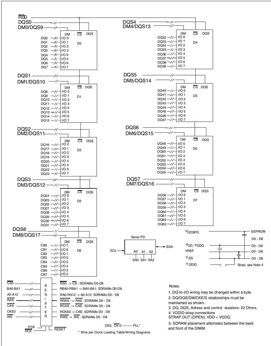
Block Diagram: One Bank 32Mb x 72 DDR-I SDRAM DIMM Module HYS72D32000GR using x8 organized SDRAMs on Raw Card Version A
