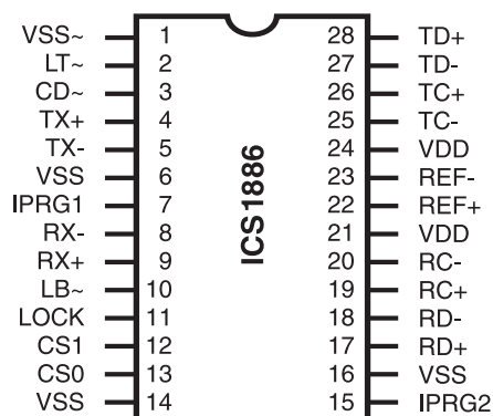
28-Pin SOIC
