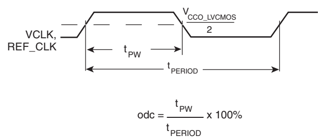
LVCMOS OUTPUT DUTY CYCLE/PULSE WIDTH/tPERIOD
