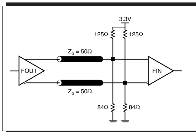
FIGURE 7B. LVPECL OUTPUT TERMININATION
