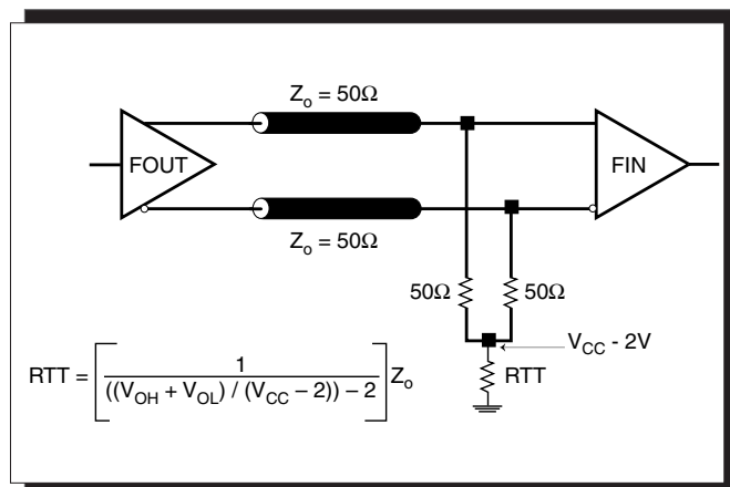
FIGURE 7A. LVPECL OUTPUT TERMININATION
