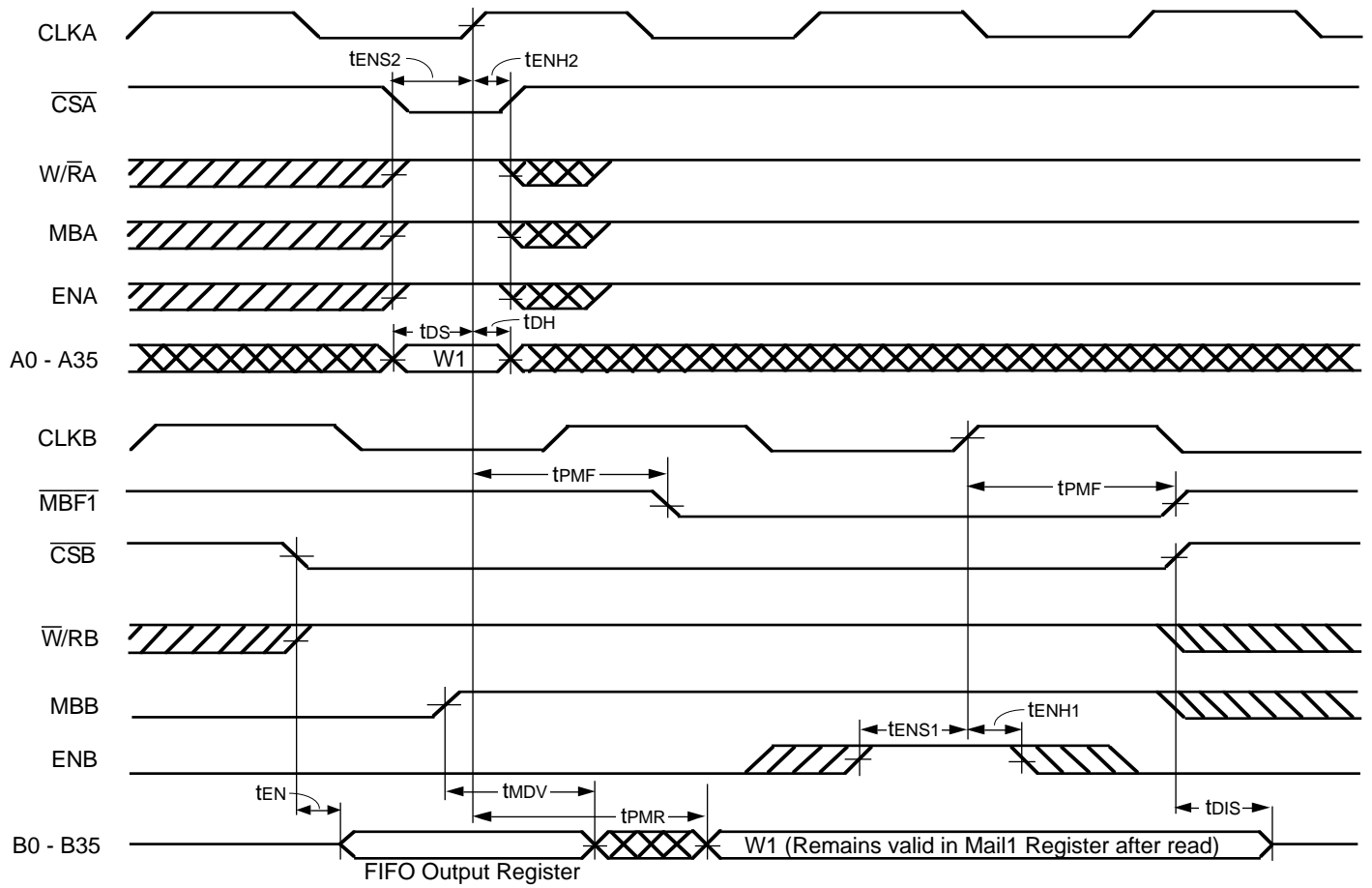
Figure 14. Timing for Mail1 Register and \overline{\text{MBF1}} Flag
