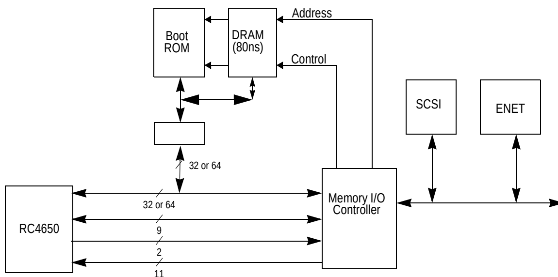
Figure 3 Typical RC4650 System Architecture
