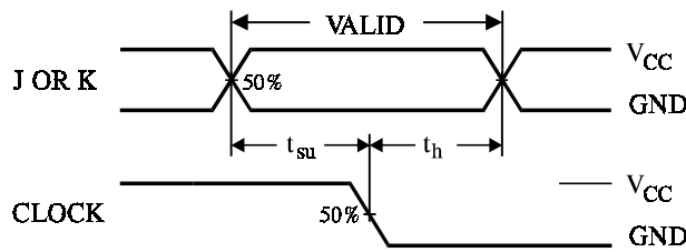
Figure 3. Switching Waveform
