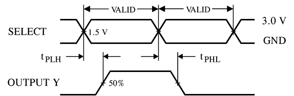
Figure 2. Switching Waveforms
