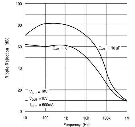
Ripple Rejection
