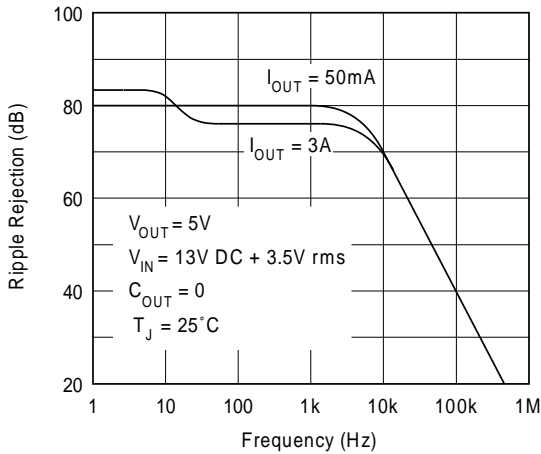
RIPPLE REJECTION
