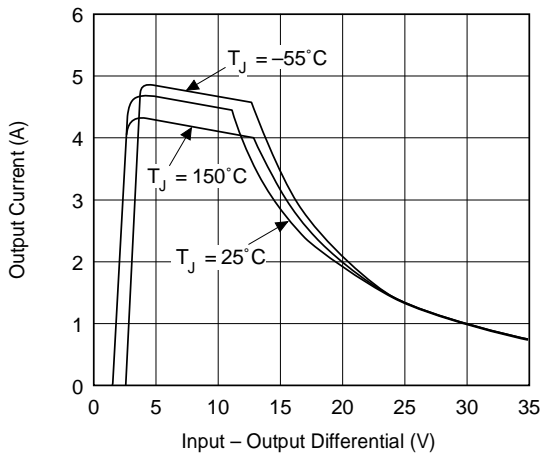
CURRENT LIMIT
