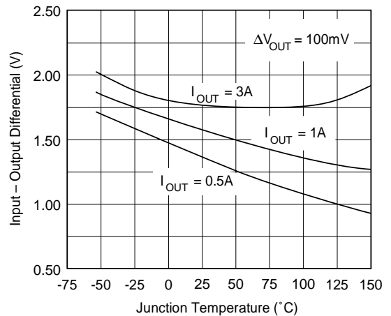
DROPOUT VOLTAGE
