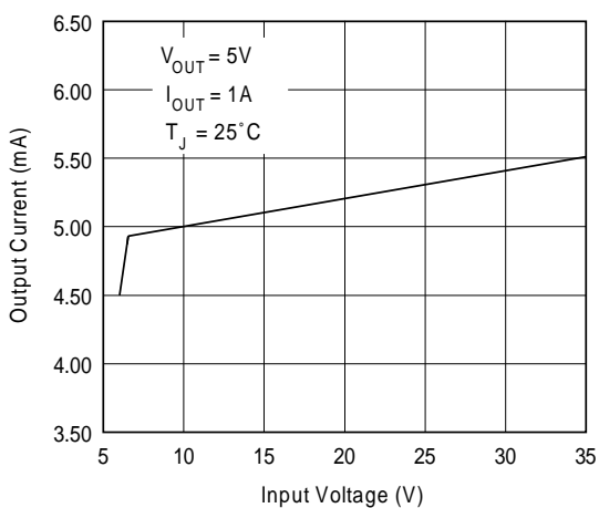
QUIESCENT CURRENT
