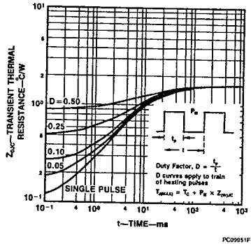
Figure 12 Transient Thermal Resistance vs Time for MTP10N08/10N10
