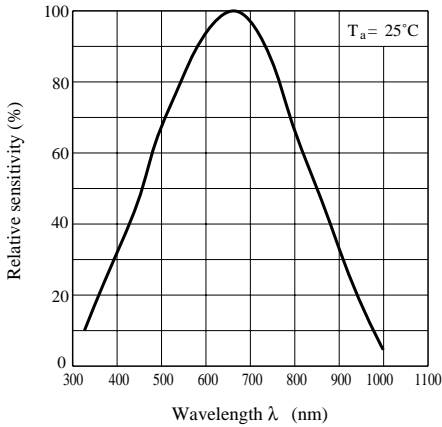
Fig. 9 Spectral Sensitivity
