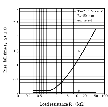
Fig. 6 Rise, Fall Time vs. Load Resistance
