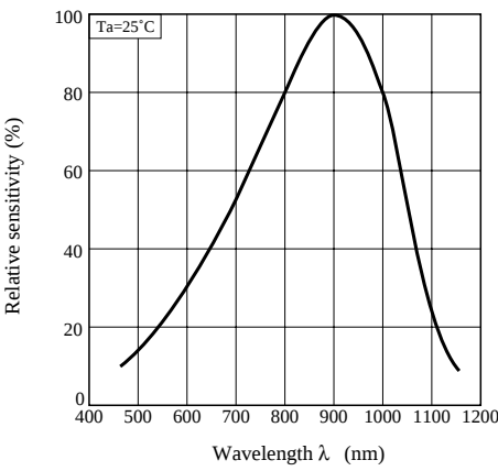
Fig. 8 Spectral Sensitivity (TYP.)
