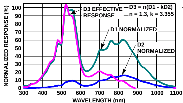
FIGURE 8. SPECTRAL RESPONSE
