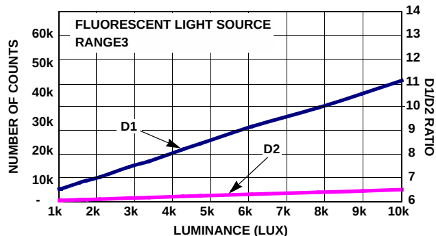
FIGURE 9. D1 AND D2 FLUORESCENT LIGHT SOURCE RESPONSE
