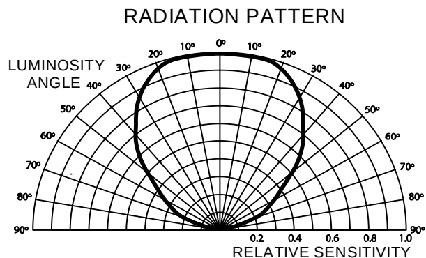
FIGURE 13. RADIATION PATTERN
