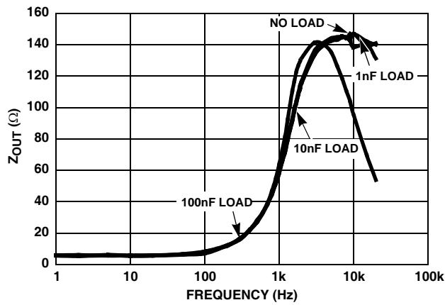
FIGURE 13. Z_{OUT} vs FREQUENCY
